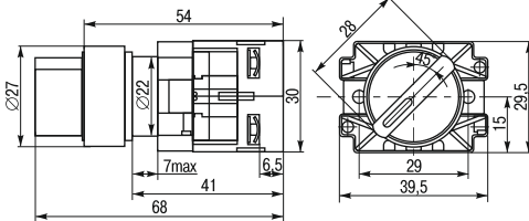
LAY5-BK2365, LAY5-BK2465, LAY5-BK2565
